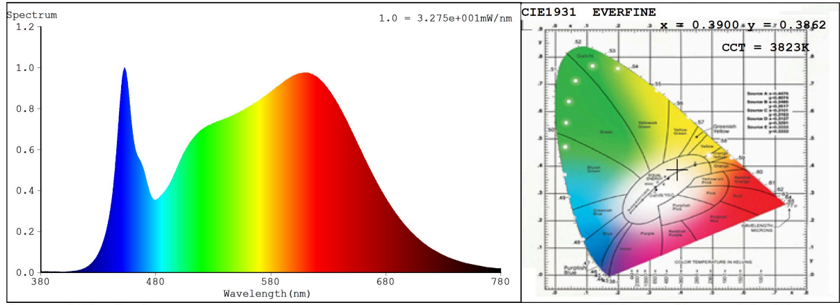
Spectral Distribution
